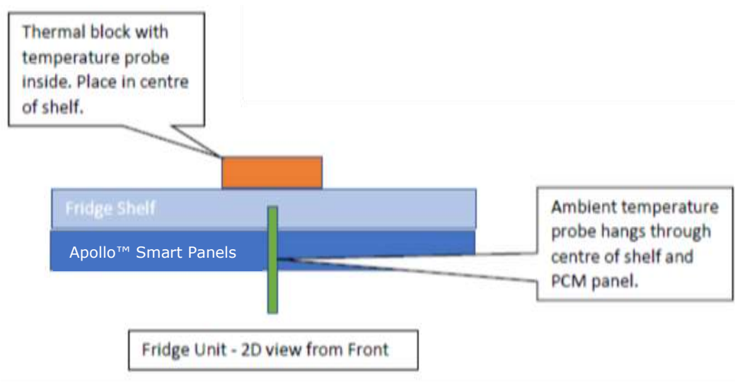
Figure 3: temp. sensors
