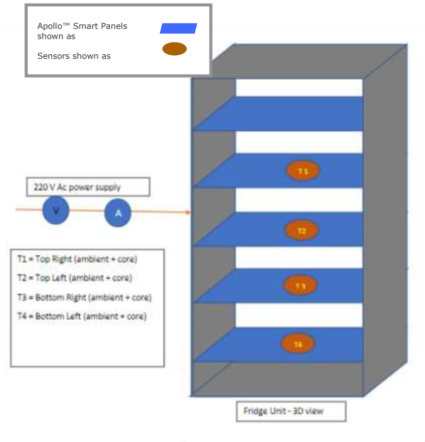
Figure 2: Fridge Schematic
